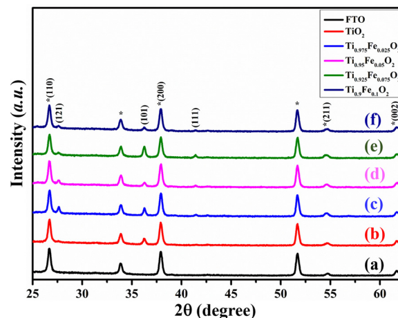
Fig. 2 XRD patterns of the (a) FTO, (b) bare TiO_2 , (c) Ti_{0.975}Fe_{0.025}O_2 , (d) Ti_{0.95}Fe_{0.05}O_2 , (e) Ti_{0.925}Fe_{0.075}O_2 , and (f) Ti_{0.9}Fe_{0.1}O_2 TiO_2 NRs, respectively. * represents FTO peaks.
