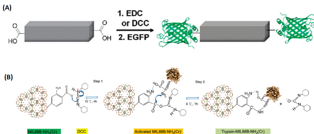
Fig. 11 The bioconjugation of proteins onto the surface of MOFs via functional groups of the organic linkers. (A) The bioconjugation of the 1D-MOFs, [(Et_2NH_2)(In(pda)_2)]_n , with EGFP. 89 Copyright 2011, Chemical Communications (Camb). (B) Trypsin immobilization onto DCC-activated MIL-88B-NH 2 (Cr). 90 Copyright 2012, ChemPlusChem .
