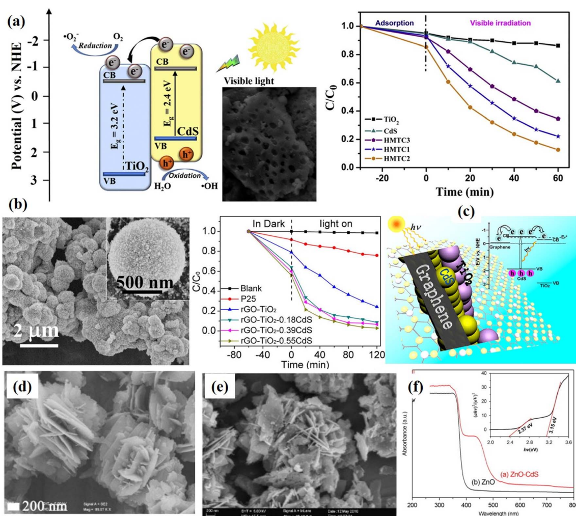
Fig. 16 (a) Hierarchically meso- and macroporous TiO 2 /CdS i.e. HMTCC heterostructure materials and its visible light photocatalytic activity for the degradation of RhB. HMTCC1, HMTCC2, HMTCC3 show different concentrations of CdS and HMTCC2 is the optimized concentration. Reprinted with permission from ref. 157 (b) rGO/TiO 2 /CdS nanocomposites and degradation efficiency of towards MB aqueous solution, reprinted with permission from ref. 26 (c) a possible reaction mechanism of charge transfer in CdS/graphene/TiO 2 hybrid nanocomposites for excellent photocatalytic activity. Reprinted with permission from ref. 160 (d–f) FESEM micrographs of ZnO and ZnO/CdS hybrid nanostructures and UV-visible absorption spectra respectively. Reprinted with permission from ref. 161.
