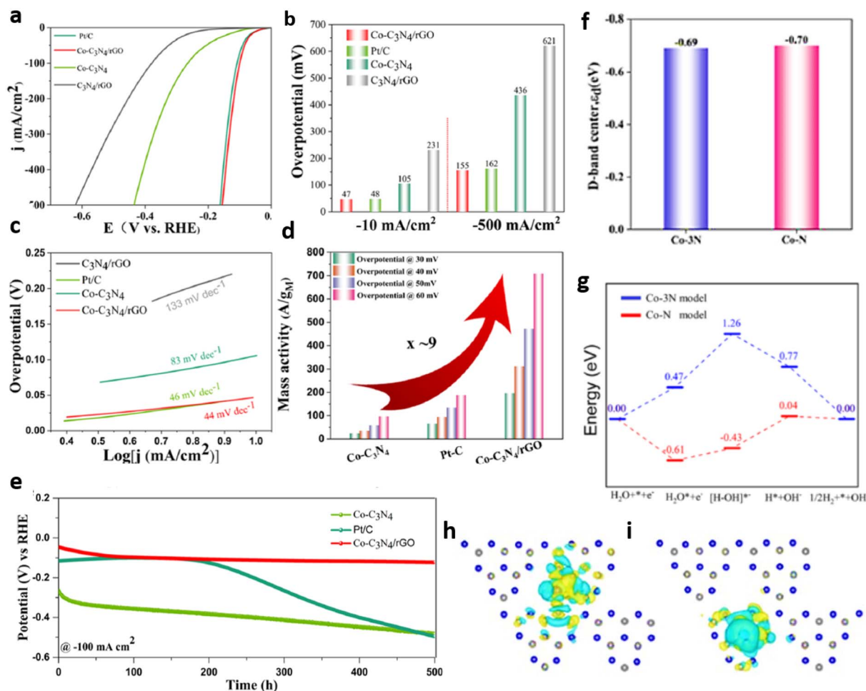
Fig. 31 Data elucidation of HER activity, (a) LSV curves in 1.0 m KOH, at a scan rate of 5 \text{ mV s}^{-1} for Co-C 3 N 4 /rGO, Co-C 3 N 4 , C 3 N 4 /rGO, and Pt/C, (b) overpotential values of the developed catalysts for a current density of -10 and -500 \text{ mA cm}^{-2} , (c) Tafel plots, (d) mass activity of the developed catalyst in comparison with Pt/C, at different overpotentials (e) time-dependent overpotential curves of Co-C 3 N 4 /rGO, Co-C 3 N 4 , in comparison with Pt/C. Co-N and Co-3N systems with (f) d-band centers, (g) energy profiles, charge density differences in structures of (h) Co-N 3 , (i) Co-N 1 . Reproduced with permission from ref. 138. Copyright 2022 American Chemical Society.
