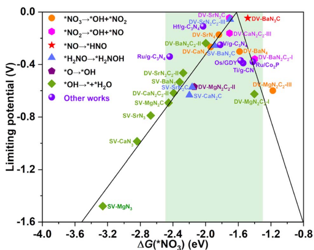
Fig. 5 The eNO 3 RR volcano diagram of the considered AE-SACs with the descriptor of \Delta G(*\text{NO}_3) . The purple spheres denote other works for comparison 45–50 . The green background encloses those AE-SACs with acceptable limiting potentials.
