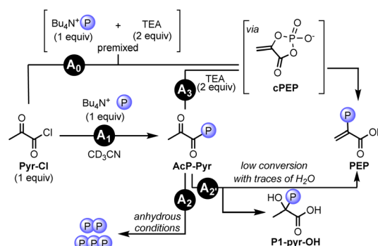
Fig. 8 Study of the phosphoryl transfer in aprotic solvent ( CD_3CN ). Reaction A 0 : reaction of premixed base and phosphate with Pyr-Cl leading to the formation of PEP through its cyclic form cPEP . Reaction A 1 : the activated carboxylic acid Pyr-Cl is transformed to the corresponding acyl-phosphate ( AcP-Pyr ), leading to the formation of polyphosphates in anhydrous conditions (A 2 ) or to the formation of PEP by either subsequent addition of TEA (A 3 ) or with trace amount of H_2O (along with the formation of the side product P1-pyr-OH (A 2' )).
