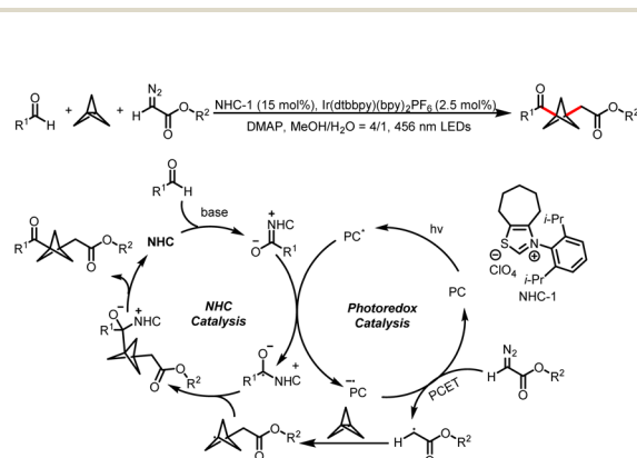
Scheme 9 Synthesis of 1,3-disubstituted bicyclo[1.1.1]pentane ketones.
