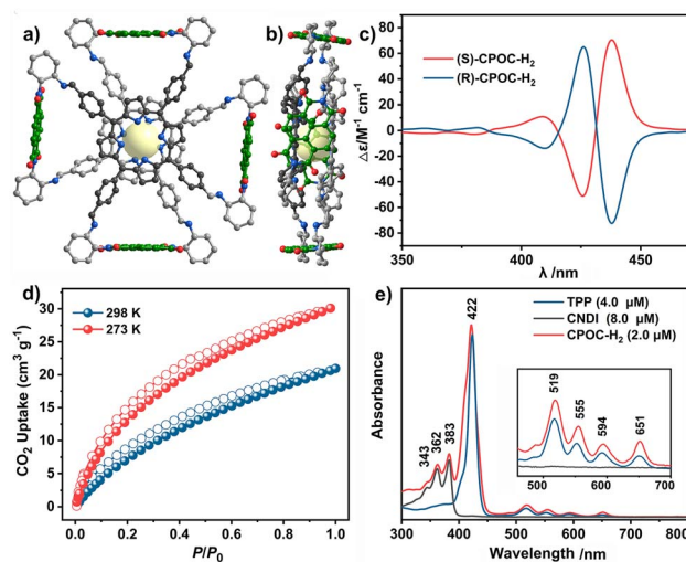
Fig. 1 Molecular structure of ( R )-CPOC-H 2 optimized by the DFT method in top (a) and side (b) view, respectively (carbon (except carbon from NDI): green; grey, nitrogen: blue, oxygen: red, central yellow ball represents void). (c) Circular dichroism spectra of ( R )-CPOC-H 2 (blue) and ( S )-CPOC-H 2 (red) in CHCl 3 . (d) CO 2 adsorption (solid) and desorption (hollow) curves of POC-H 2 at 298 K (blue) and 273 K (red). (e) Comparison of the UV-vis spectra of CPOC-H 2 and the corresponding monomeric references in CHCl 3 (inset: the enlarged spectrum from 460 to 700 nm).
