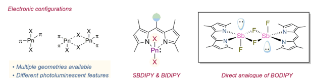
Fig. 1 Context of the work. (A) BODIPY chromophores (B) previous heavier BODIPY analogues. (C) Synthesis and characterisation of SBDIPY and BIDIPY.
