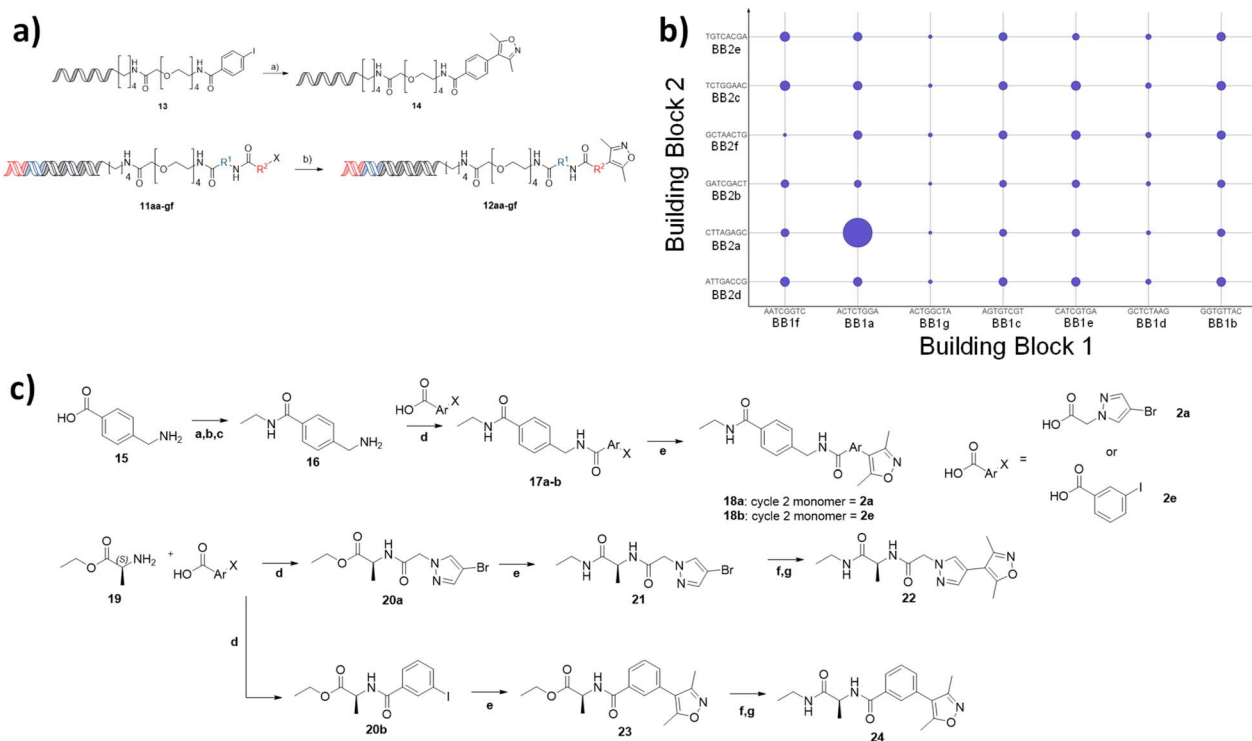
Fig. 3 (a) Coupling of the isoxazole fragment to a model substrate, showing confirmation of Suzuki coupling on DNA, and coupling to the full NUDEL, reagents: (a) Pd(dtbpf)Cl 2 , K 3 PO 4 , H 2 O/THF, TPGS-750M 2.5%, 3,5-dimethyl-4-(4,4,5,5-tetramethyl-1,3,2-dioxaborolan-2-yl)isoxazole, (b); (j) Pd(dtbpf)Cl 2 , 2% TPGS-750-M, K 3 PO 4 , H 2 O/THF; (b) Selection of targeted library against BRD4 showing enrichment of sequences by size of the points, broken down by building block 1 (X-axis) and building block 2 (Y-axis) codons; (c) Off-DNA synthesis of 4 compounds. 18a synthesised from 2a , 18b synthesised from 2e . Reagents: (a) TFAA; (b) SOCl 2 ; (c) NH 2 Et in THF 2M; (d) HATU, DIPEA, DCM (e) Pd(dtbpf)Cl 2 , Cs 2 CO 3 , Diox./H 2 O 10 : 1, 3,5-dimethyl-4-(4,4,5,5-tetramethyl-1,3,2-dioxaborolan-2-yl)isoxazole; (f) LiOH, THF/H 2 O 1 : 1; (g) HATU, DIPEA, DCM, NH 2 Et in THF 2 M.
