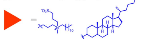
Fig. 2 General strategies for designing organelle-targeting ratiometric fluorescent probes and common organelle-targeting groups for (a) mitochondria; (b) lysosome; (c) endoplasmic reticulum; (d) Golgi apparatus; (e) nucleus; (f) membrane.
