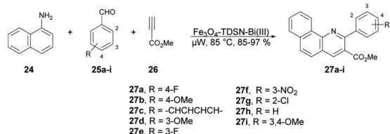
Scheme 9 Synthesis of various quinolines 27a–i.
