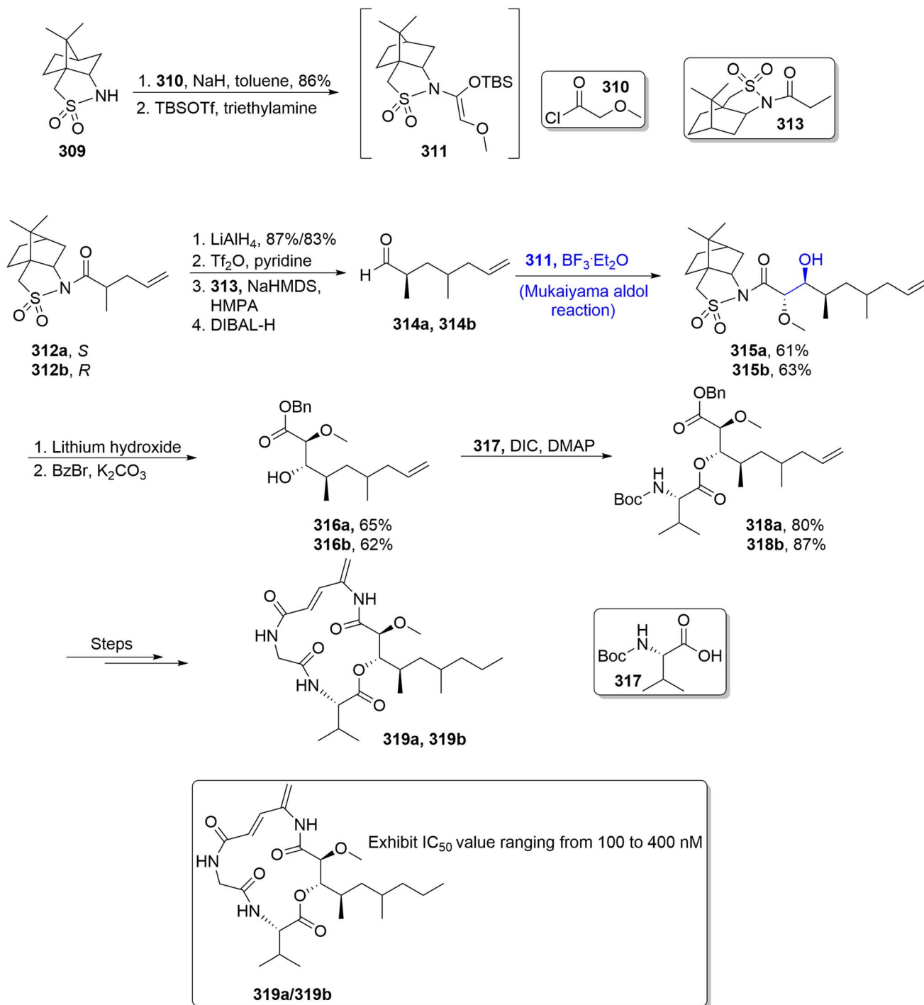
Scheme 42 Synthesis of bohohamide A 319.
