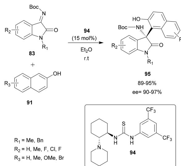
Scheme 24 Enantioselective aza-FC reaction of β-naphthol with ketamine using a Takemoto catalyst.
