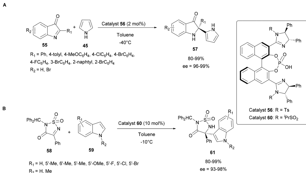
Scheme 16 Organocatalytic enantioselective aza-FC reactions using imidazolines/pyrroles and 3 H -indol-3-ones (A) or cyclic ketimines (B).
