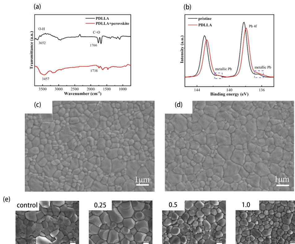
Fig. 6 (a) Fourier transform infrared spectroscopy (FTIR) spectra of polymer and cross-linked perovskite film. (b) X-ray photoelectron spectroscopy (XPS) of the Pb 4f orbital of \text{MAPbI}_3 without and with polymer integration. The SEM images of (c) pristine and (d) optimized films. The scale bar is 1.0 \mu\text{m} . Reproduced from ref. 83 with permission from Springer Nature, copyright 2022. (e) SEM images of \text{CsPbI}_2\text{Br} films modified with different PEG concentrations: control, 0.25 \text{ mg mL}^{-1} , 0.5 \text{ mg mL}^{-1} , 1.0 \text{ mg mL}^{-1} . The scale bar is 500 \text{ nm} . Reproduced from ref. 84 with permission from Elsevier, copyright 2021.
