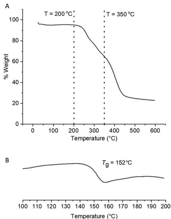
Fig. 3 For the O -methyl carbamate functionalised polymer product derived from P(Am-co-DMAm) containing 50 mol% Am; (A) TGA analysis showing two thermal events occurring between T = 200 – 350\text{ °C} and a third event at T > 350\text{ °C} ; (B) DSC analysis showing that T_g = 152\text{ °C} , decreasing from 178\text{ °C} following eHofmann rearrangement (Fig. S14†).
