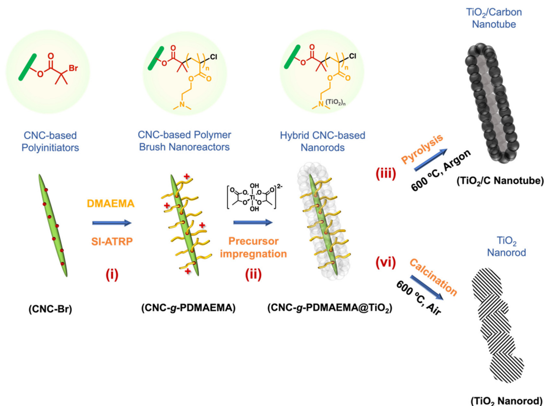
Scheme 1 Template-directed formation of anatase \text{TiO}_2/\text{carbon} nanotubes using CNC-based polymer nanoreactors.
