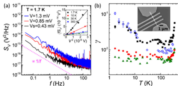
Fig. 17 (a) S_V vs. f and T for an \text{IrO}_2 NW with L = 0.9 \mu\text{m} and d = 147 \text{ nm} ; \langle S_V \rangle vs. V^2 is shown in the inset. (b) \gamma = S_V N_c f / V^2 vs. T for \text{IrO}_2 NWs from 1.7 K to 350 K. The inset is a SEM image of a NW. Dimensions are L = 1.9 \mu\text{m}, d = 143 \text{ nm} (solid black squares); L = 1.0 \mu\text{m}, d = 123 \text{ nm} (solid green triangles); and L = 0.9 \mu\text{m}, d = 147 \text{ nm} (open blue diamonds). Reproduced from ref. 75 with permission. Copyright 2023 American Institute of Physics.
