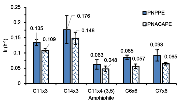
Fig. 4 Rate constants of PNPPE (blue, solid fill) and PNCAPE (blue, shingle pattern) depropargylation in presence of C11×3, C14×3, C11×4 (3,5), C6×6 and C7×6 metallic micelles.
