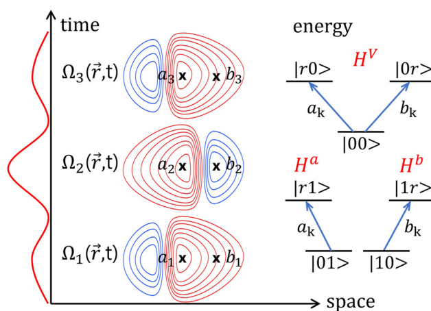
Fig. 1 Proposed implementation of the SOP for two-qubit gates. The qubits are located at the x positions. They are subject to the pulses, \Omega_1(\vec{r}, t) , \Omega_2(\vec{r}, t) , \Omega_3(\vec{r}, t) whose spatial profile is shown in the horizontal “space” axis, with local amplitudes at the qubits designated by the geometrical factors a_k and b_k . Different colors represent a \pi phase change in the amplitude of the field (red – positive; blue – negative). The sequence of operations that governs the temporal evolution of the state vectors depends on the pulse sequence, shown in the vertical “time” axis. Conditional on the initial state of the qubit, |00\rangle , |01\rangle , |10\rangle , the energy diagram of the subsystem where the dynamics takes place is shown under “energy”. The |11\rangle , not shown, is completely decoupled.
