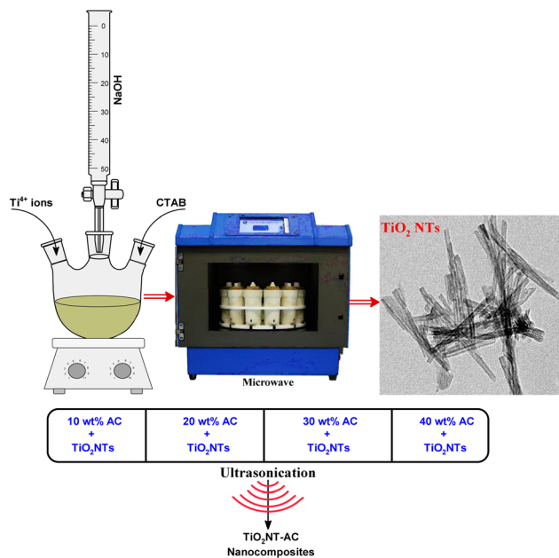
Scheme 1 Synthesis of \text{TiO}_2 NTs and ultrasonic deposition of AC on \text{TiO}_2 NTs.
