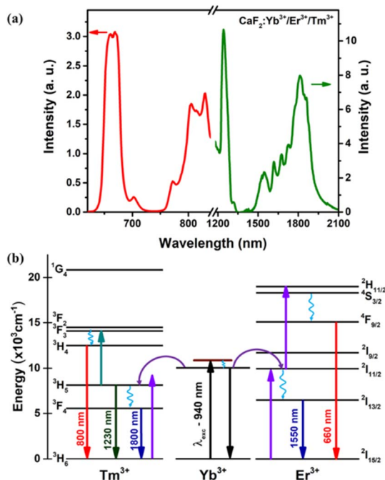
Fig. 5 (a) Emission spectrum of \text{Yb}^{3+}/\text{Er}^{3+}/\text{Tm}^{3+} tri-doped \text{CaF}_2 NPs under 940 nm excitation at room temperature in the I-BW (red) and III-BW (left peak of the green spectrum) and III-BW (right peak of the green spectrum). (b) Simplified energy scheme of the \text{Yb}^{3+} , \text{Er}^{3+} and \text{Tm}^{3+} ions, showing excitation and emission decays (full lines), nonradiative decays (wavy lines), and the energy transfer process (curved lines).
