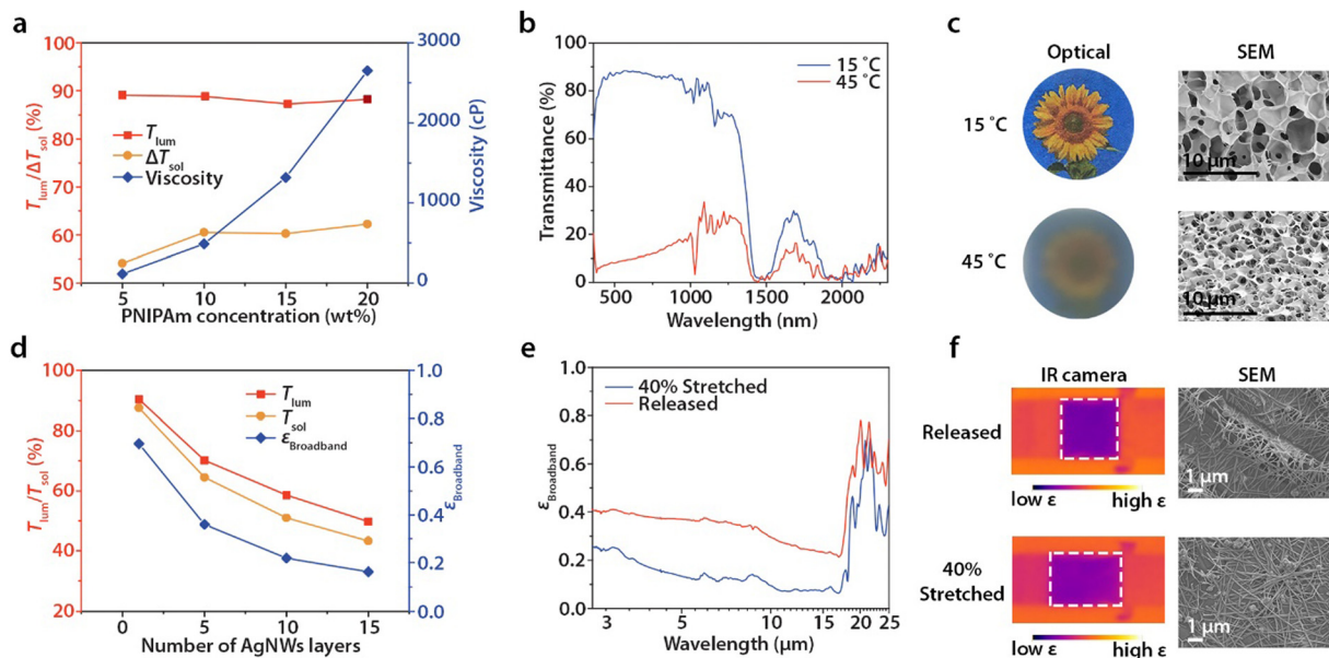
Fig. 2 (a) Thermochemical properties for the hydrogel composite and viscosity of monomer ink with different PNIPAm concentrations. (b) UV-Vis-NIR spectra for 10 wt% PNIPAm hydrogel at 15 °C and 45 °C. (c) The photo and SEM image of the smart hydrogel at 15 and 45 °C. (d) The T_{lum} , T_{sol} , and integrated \epsilon_{Broadband} for the PDMS film with different layers of coatings of AgNWs. (e) The broadband emissivity spectra of the 15-layer AgNWs-coated PDMS film in its released and 40%-stretched states. (f) IR camera images and SEM images for the 15-layer AgNWs-coated PDMS film in its released and 40%-stretched states.
