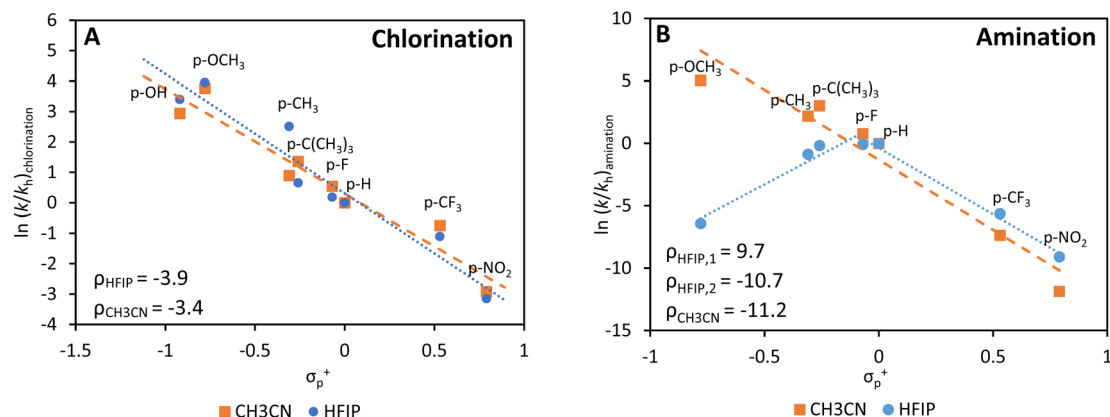
Fig. 5 Hammett plots of the homogeneous chlorination (A) and amination (B) reaction in HFIP and \text{CH}_3\text{CN} . Only the product with the \text{Cl}^- or amino-substituent on the para position is considered in these plots. Reaction conditions: 0.1 mmol piperidine, 1 equiv. NCS, 18 equiv. arene, 4 equiv. \text{HClO}_4 , 1 mL HFIP or \text{CH}_3\text{CN} , 2 mol% \text{Ru}(\text{bipy})_3\text{Cl}_2 , 15 min, R.T.
