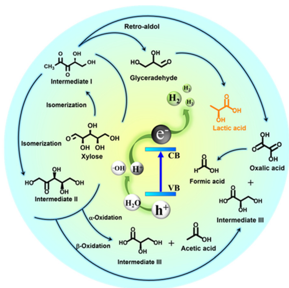
Fig. 8 Possible reaction mechanism of the photocatalytic co-production of hydrogen and lactic acid via \text{RuS}_2@CN-2 .
