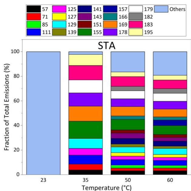
Fig. 4 Evolution of VOC emission composition in % for the 20 masses exhibiting the strongest contributions ( EF > 22 \mu\text{g m}^{-2} \text{h}^{-1} at 60 °C) as a function of temperature, as measured by PTR-ToFMS under dry ( RH = 0.1\% ) and dark conditions, for the STA3 fresh asphalt sample.
