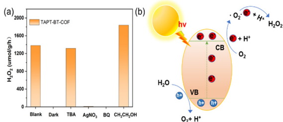
Fig. 6 Mechanism studies. (a) Photocatalytic H 2 O 2 production of TAPT-BT-COF under different conditions. (b) Schematic diagram of the catalytic reaction mechanism.
