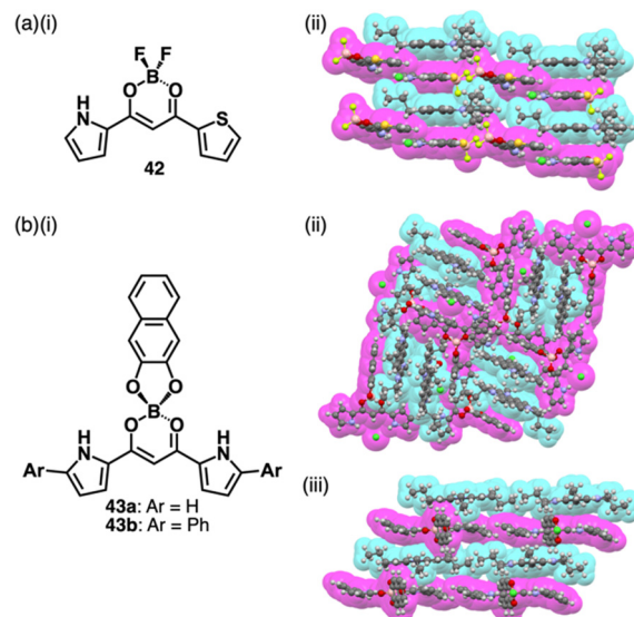
Fig. 29 (a) (i) Pyrrolylthienyldiketone BF_2 complex 42 and (ii) single-crystal X-ray structure of {}^3TATA^+ \cdot 42_2 \cdot Cl^- and (b) (i) naphthalenediolate boron complexes 43a,b and (ii) single-crystal X-ray structures of {}^3TATA^+ \cdot 43a \cdot Cl^- and (iii) {}^3TATA^+ \cdot 43b \cdot Cl^- . The crystal structures are redrawn from cif files: 1840326, 2227398 and 2227399.
