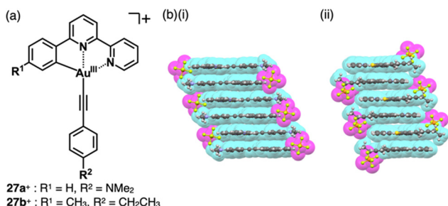
Fig. 17 (a) Positively charged phenylbipyridine Au III complexes 27a,b + and (b) single-crystal X-ray structures of (i) 27a + -PF 6 - and (ii) 27b + -PF 6 - (redrawn from cif files: 841764 and 897336).
