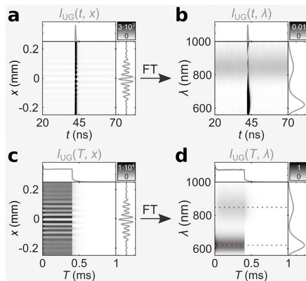
Fig. 2 Ungated bmFIS data of (\text{DNA})_2[\text{Ag}_{18}]^{12+} in an aqueous solution at RT with 520 nm excitation ( I = 3.4 \text{ kW cm}^{-2} , f_{\text{Micro}} = 13 \text{ MHz} , f_{\text{Macro}} = 1 \text{ kHz} , T_{\text{on}} = 0.4 \text{ ms} , T_{\text{off}} = 0.6 \text{ ms} ). Micro-time domain (a) TRIM and (b) TREM. Macro-time domain TRIM (c) and TREM (d). The blue and red dashed lines in (d) indicate the maxima of the long- and short-lived bands, respectively.
