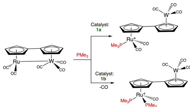
Scheme 2 ETC-catalyzed \text{PMe}_3 ligand addition in the fulvalene heterobimetallic complex [\text{RuW}(\eta^{10}\mu^2\text{-C}_{10}\text{H}_8)(\text{CO})_5] . The reaction depends on the \text{Fe(II/I)} redox potential of the electron-reservoir ETC catalyst ( 1a vs. [\text{Fe}(\eta^5\text{-C}_5\text{Me}_5)(\eta^6\text{-C}_6\text{Me}_6)] , 1b ). With the more electron-rich electron reservoir 1b as ETC catalyst, two \text{PMe}_3 ligands are introduced whereas, with 1a , only one \text{PMe}_3 ligand is added. ETC catalysis was pioneered by Henry Taube. 27
