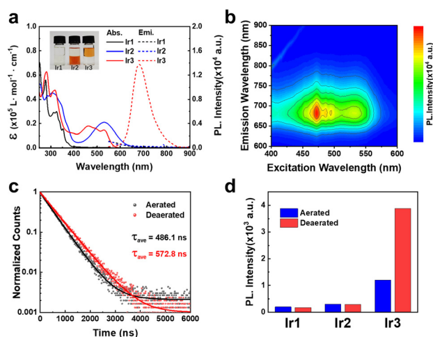
Fig. 1 (a) UV-Vis absorption and emission spectra of Ir1–Ir3 in \text{CH}_2\text{Cl}_2 at room temperature. Insert: Log P o/w of Ir1–Ir3 (b) 3D mapping phosphorescence spectra of the Ir3 (10 \mu\text{M} ) in \text{CH}_2\text{Cl}_2 at room temperature. (c) Phosphorescence lifetime of Ir3 in \text{CH}_2\text{Cl}_2 under air or N 2 . (d) Phosphorescence intensity of Ir1–Ir3 (10 \mu\text{M} ) in \text{CH}_2\text{Cl}_2 .
