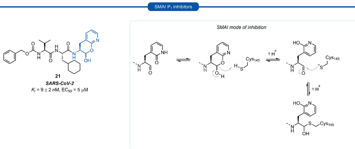
Scheme 2 Putative mechanism of reversible covalent inhibition of a cysteine protease by SMAIs.
