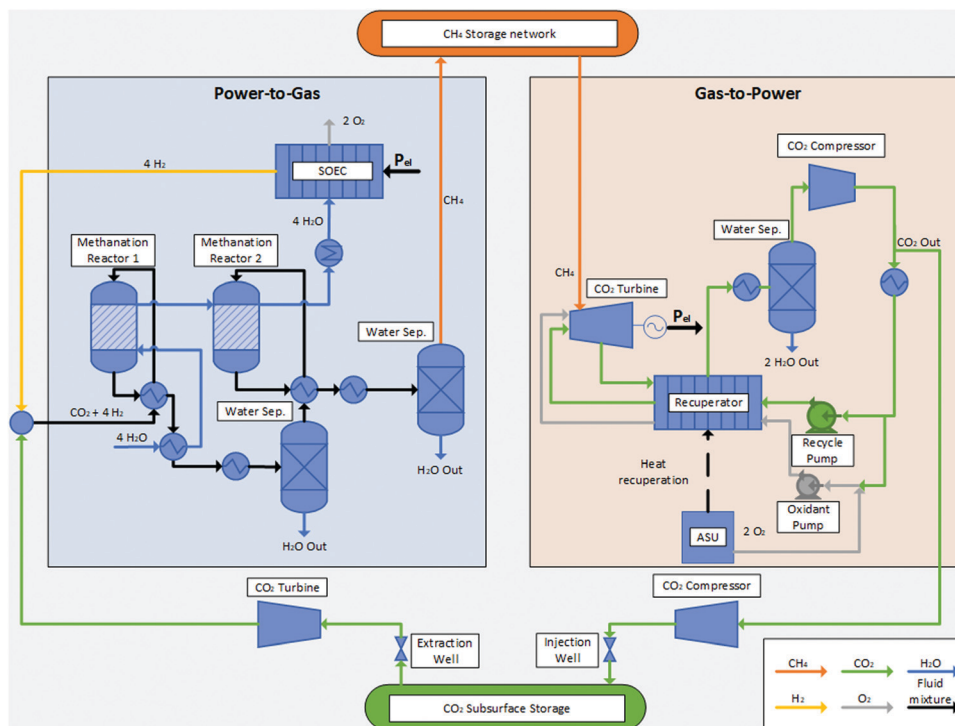
Fig. 2 Flow chart of the combined PtG-GtP and subsurface storage energy plant.
