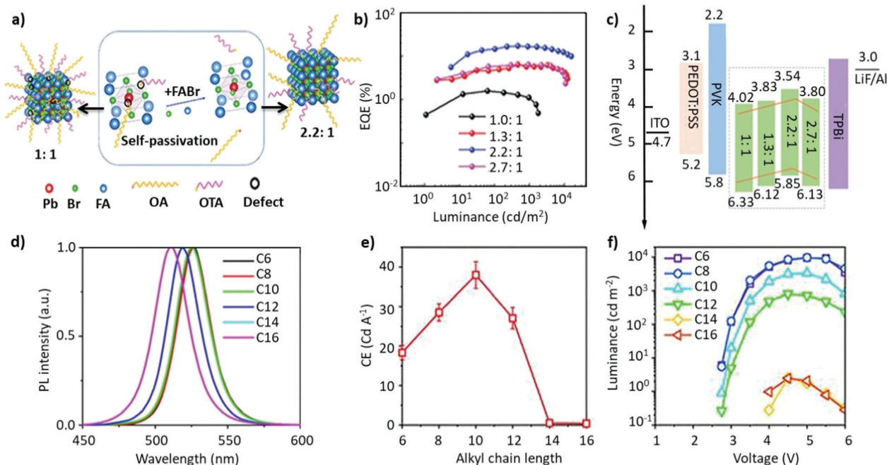
Fig. 11 (a) Reaction illustrating the self-passivation of excess FABr . (b) EQE–luminance curves of PeLEDs based on FAPbBr_3 NCs with varying molar ratios of FABr/PbBr_2 . (c) Energy-band diagram of FAPbBr_3 NCs with varying molar ratios of FABr/PbBr_2 . (d) PL emission spectra of FAPbBr_3 NCs synthesized using various chain lengths of alkylamine ligands, (e) current efficiency as a function of the alkyl chain length, and (f) luminance–voltage curves for PeLEDs with different chain lengths (from C6–C16). Panels (a–c) adapted from ref. 125. Copyright 2020 WILEY-VCH Verlag GmbH & Co. KGaA, Weinheim. Panels (d–f) reproduced with permission from ref. 193. Copyright 2019 American Chemical Society.
