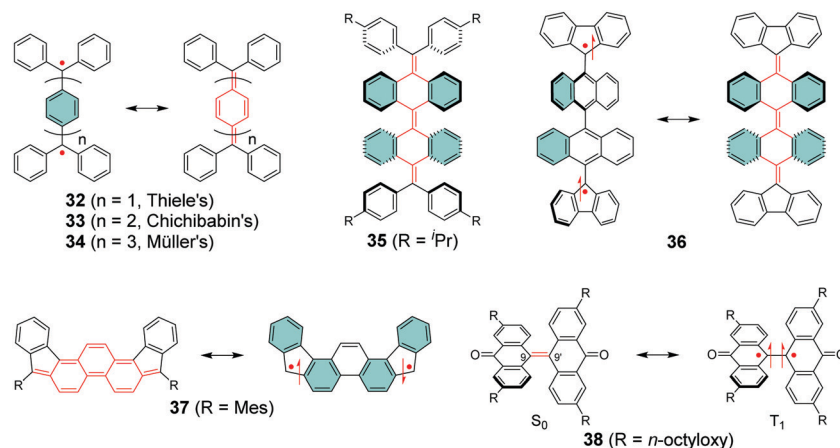
Scheme 9 Closed-shell and open-shell resonance structures of Thiele's, Chichibabin's and Müller's hydrocarbons and related derivatives (R groups are omitted from some resonance structures for clarity).
