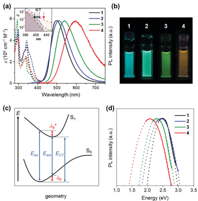
Fig. 3 (a) UV-vis absorption and PL spectra of 1 – 4 in toluene ( 1 \times 10^{-5} M). The inset shows a magnified view of the ICT absorption bands. (b) Photograph of the PL emissions from the solutions under UV irradiation. (c) Schematic potential energy diagram of the S_0 and S_1 states; E_{ex} , E_{em} , and E_{CT} denote the energies of excitation, emission, and charge transfer, respectively. (d) PL spectra (solid lines) fitted using eqn (1) for the evaluation of \lambda_S .
