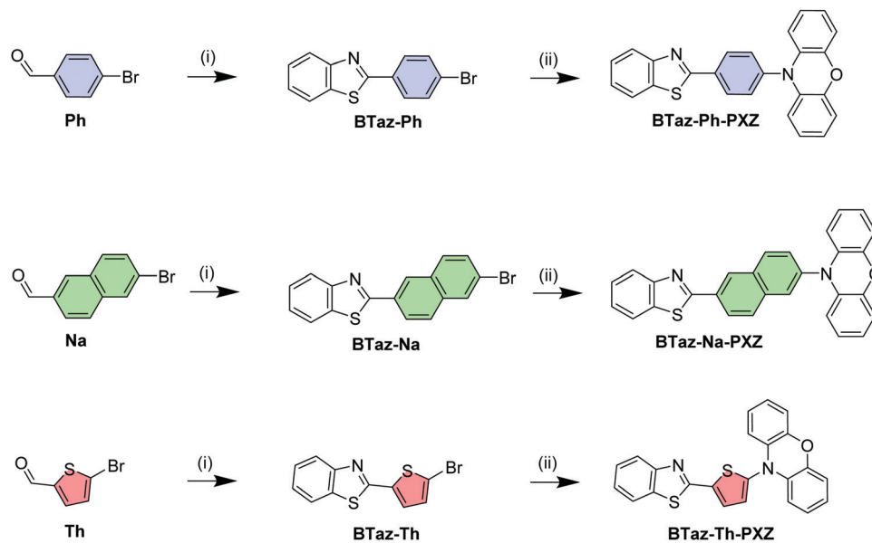
Scheme 1 Synthesis procedures for the three BTaz-Ar-PXZ emitters: (i) 2-aminothiophenol, sodium metabisulfite, DMF, reflux, 2 h; (ii) Pd(OAc) 2 , 10 H -phenoxazine, (t-Bu) 3 P, N iBuO, toluene, reflux, 16 h.
