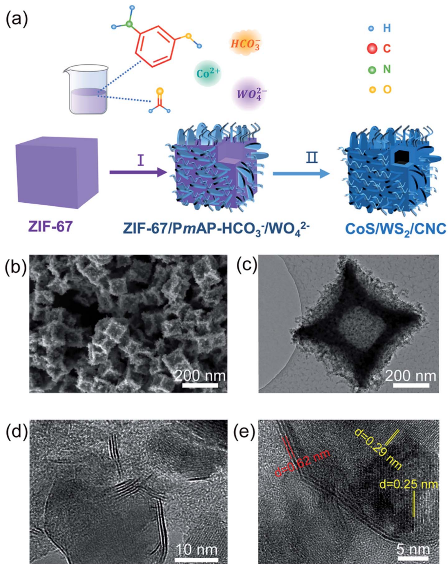
Fig. 1 (a) Schematic illustration of the fabrication pathway of CoS/WS 2 /CNC. (b) SEM, (c) TEM, and (d) TEM, and (e) high-resolution TEM images of CoS/WS 2 /CNC-1.
