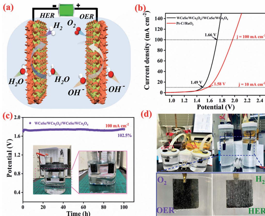
Fig. 5 Electrochemical performance of the water splitting cell in an alkaline medium: (a) illustration of the electrochemical water splitting device, (b) LSV curves of the WCoSe/WCo 3 O 4 /WCoSe/WCo 3 O 4 and Pt-C/RuO 2 -NF devices in 1.0 M KOH, (c) long-term stability test of the WCoSe/WCo 3 O 4 /WCoSe/WCo 3 O 4 electrochemical water splitting device at a current density of 100 mA cm -2 over 100 h (inset shows the generation of H 2 and O 2 during the electrocatalytic process), and (d) the setup measurement of H 2 and O 2 generation during water electrolysis.
