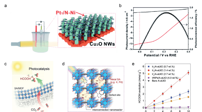
Fig. 6 (a) Schematic illustration and (b) PEC performance of Pt 1 /N–Ni/Cu 2 O NWs for water reduction. 24 Reproduced with permission from ref. 24. Copyright 2021, The Royal Society of Chemistry. The scheme of (c) MOF membrane and (d) MOF structures with single metal atoms for photocatalytic CO 2 reduction. (e) Time course of HCOOH evolution on A-aUiO, Ir 1 /A-aUiO, Ir x /A-aUiO and IrNPs/A-aUiO catalysts. 74 Reproduced with permission from ref. 74. Copyright 2021, Springer Nature.
