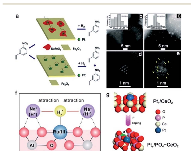
Fig. 6 (a) The proposed mechanism for hydrogenation of 3-nitrostyrene over Na-containing and Na-free Pt/FeO x catalysts. HAADF-STEM images of (b and d) 2.16% Pt/FeO x and (c, e) 5.03% Na to 2.16% Pt/FeO x . Reproduced from ref. 92, under terms of Creative Commons license, Published 2017 by Royal Society of Chemistry. (f) Schematic diagram of the role of Na + cations in stabilizing the Ru(III) species. Reproduced with permission from ref. 93. Copyright 2020, Springer Nature. (g) Schematic illustration of the formation of Pt 1 /PO 4 –CeO 2 by P doping. Reproduced with permission from ref. 94. Copyright 2019, American Chemical Society.
