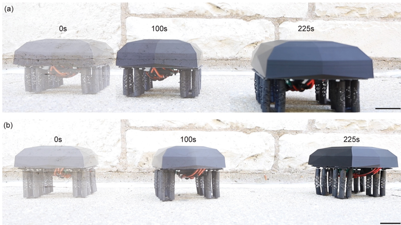
Fig. 6 Untethered soft robotic quadrupeds. Untethered HSA-based soft robots constructed with the (a) 0.5 \times legs and (b) stilted 0.5 \times legs are shown walking on a concrete sidewalk. Overlays of the quadrupeds are shown at 0 s, 100 s, and 225 s of the walking sequence. Stills are taken from Movie S4 in the ESI.† Scale bars are 50 mm.
