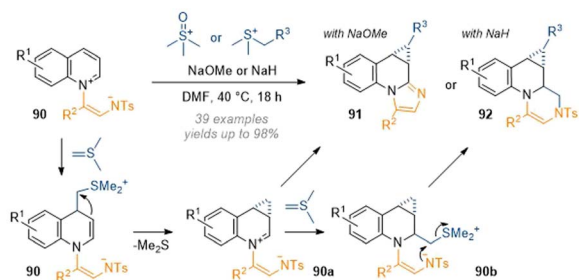
Scheme 26 Cyclopropanation of activated quinolines to form tetracycles. 32
