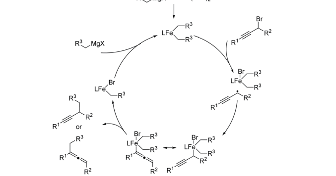
Scheme 22 Fe-catalyzed radical synthesis of allenes from propargyl bromides.
