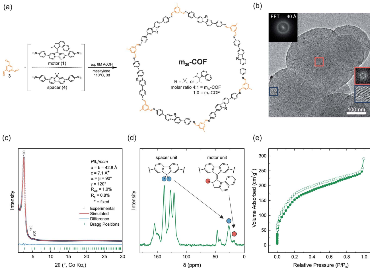
Fig. 2 (a) Synthesis of m_{20} -COF from mixtures of spacer and motor building blocks with triformylbenzene (3) under solvothermal conditions. (b) Transmission electron microscopy (TEM) image of m_{20} -COF with visible pore channels along [00 l ] pointing towards the surface of the spherical particle (blue inset). Fast Fourier transformed (FFT) insets show a hexagonal pattern (red box, viewing direction [00 l ]). (c) XRPD pattern and unit cell parameters of m_{20} -COF obtained by Pawley refinement with a simplified unit cell proxy model (see Table S1 ^\dagger ) (d) ^{13}\text{C} -CPMAS ssNMR spectrum of m_{20} -COF containing signals of the motor and spacer building blocks. (e) \text{N}_2 adsorption isotherm of m_{20} -COF.
