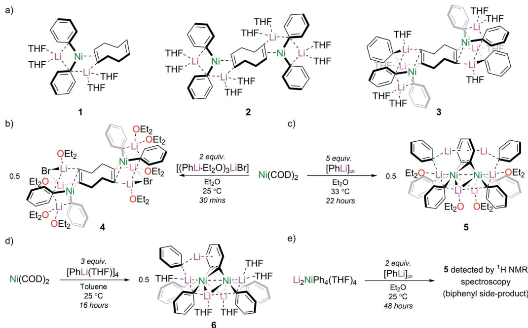
Fig. 1 (a) Lithium nickelates (1–3) derived from Ni(COD) 2 and PhLi; (b) synthesis of [Li 2 (Et 2 O) 4 (LiBr)Ph 2 Ni] 2 COD (4); (c) synthesis of [(Li 2 (Et 2 O) 4 (LiBr)Ph 2 Ni) 2 (μ-η 2 :η 2 -C 6 H 4 )] (5); (d) synthesis of heptametallalithium nickelate 6; (e) observation of 5 by reduction of Li 2 NiPh 4 (THF) 4 .
