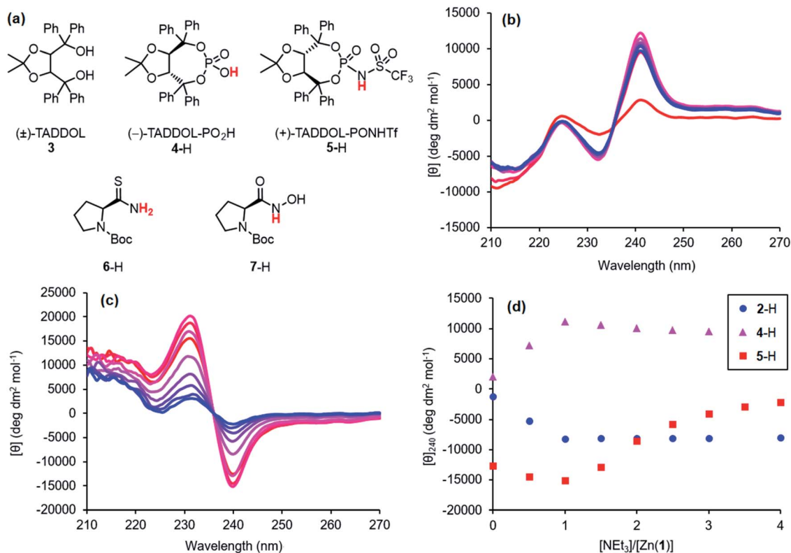
Fig. 3 (a) Structures of 3 and ligands 4–7 ; CD spectra of Zn(1)·2ClO 4 ( c_0 = 0.25 mM) with (b) 4-H (1 eq.) or (c) 5-H (1 eq.) in MeCN with addition of \text{NEt}_3 (0.0 \rightarrow 4.0 eq.) in 0.5 eq. increments; (d) molar ellipticities at 240 nm of Zn(1)·2ClO 4 ( c_0 = 0.25 mM) and 2-H , 4-H or 5-H (1 eq.) with addition of \text{NEt}_3 .
