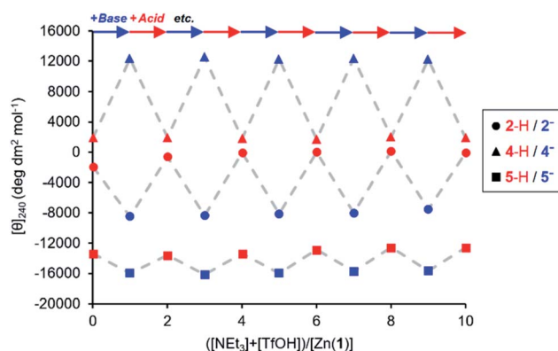
Fig. 4 Molar ellipticities at 240 nm of \text{Zn}(\mathbf{1})\cdot 2\text{ClO}_4 ( c_0 = 0.25 mM) with 2-H , 4-H or 5-H (1 eq.) in MeCN with alternating addition of \text{NEt}_3 ( \rightarrow ) and TfOH ( \rightarrow ) in 1 eq. increments.
