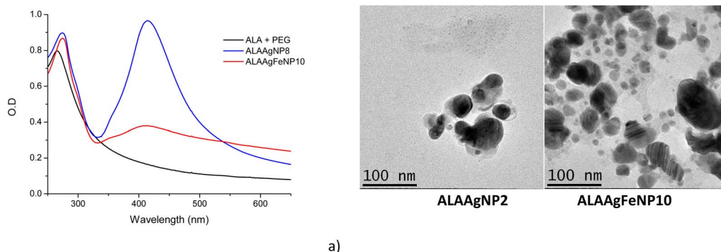
Fig. 2 (a) UV-vis spectra of ALA, ALAAgNP8 and ALAAgFeNP10. (b) TEM image of the samples: ALAAgNP2 and ALAAgFeNP10.
