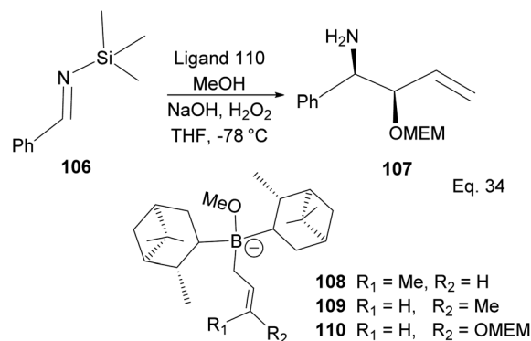
Scheme 30 Allylation and crotyllalylboration of silylaldimine.
