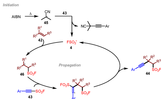
Scheme 8 Radical difunctionalization of unactivated alkenes to access \beta -alkynyl-fluorosulfonylalkanes.
