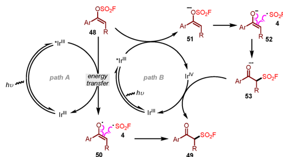
Scheme 9 Synthesis of \beta -keto sulfonyl fluorides via photocatalytic transformation of vinyl fluorosulfates.
